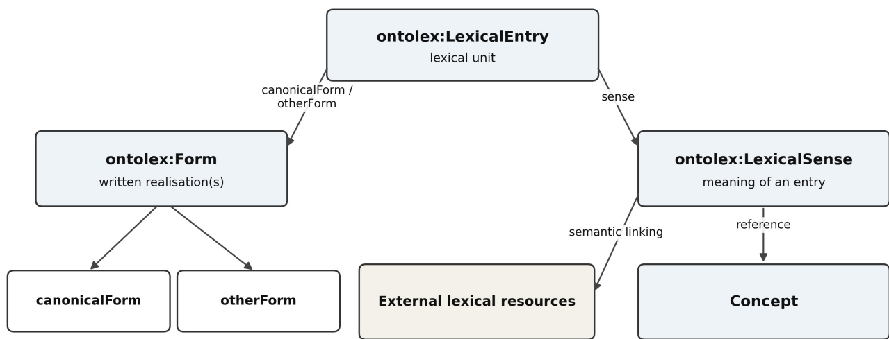
Figure 1. Simplified representation of the core OntoLex-Lemon components used in ITALMUD.
