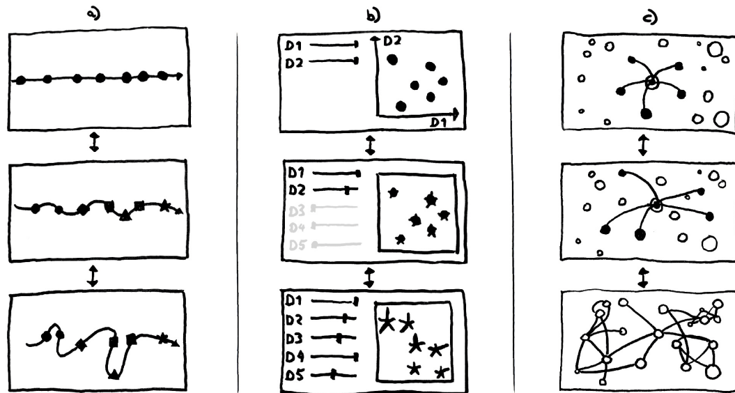
Figure 3. Examples of complication: a) Folding of a timeline based on similarity between data points. b) Use of multidimensional reduction techniques in combination with encoded glyphs for gradual addition of more dimensions in two-dimensional displays. c) Switching between egocentric and noncentric total states of a node-link network graph.
