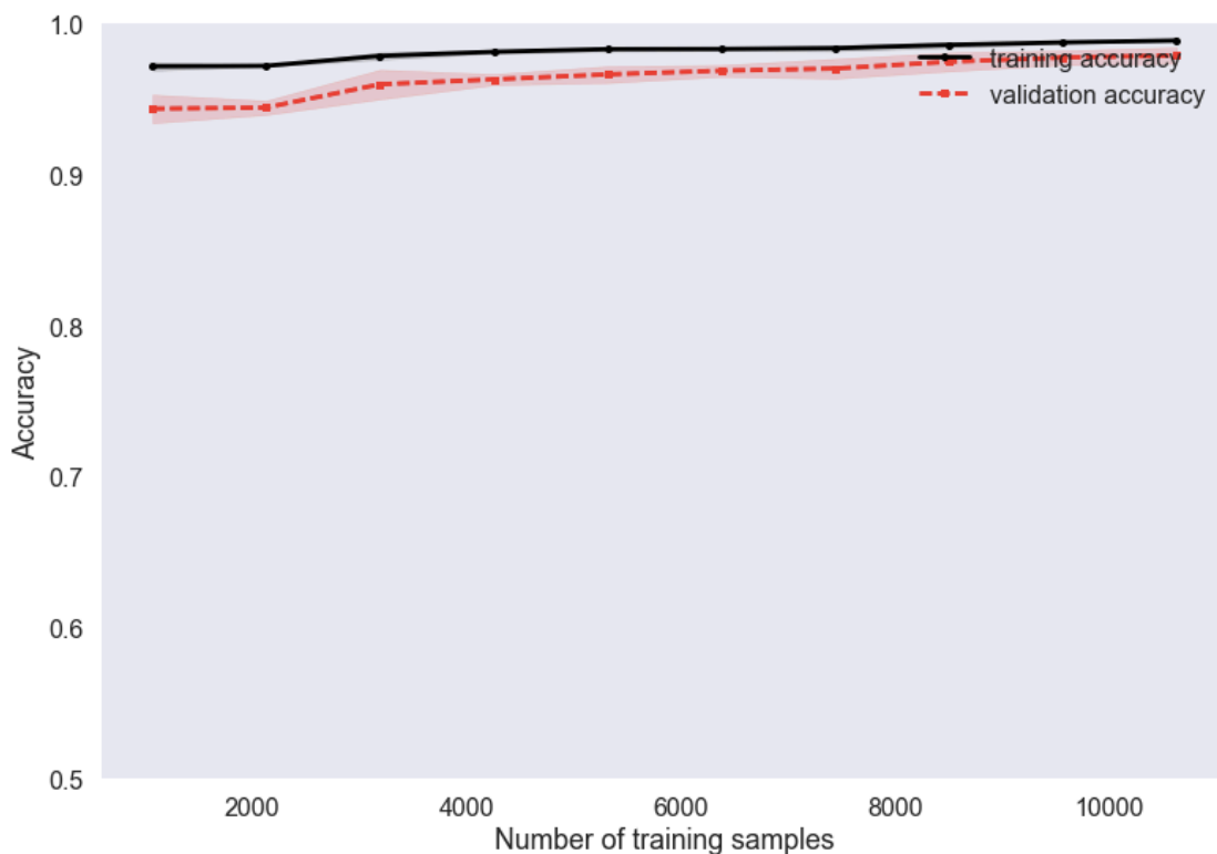
Figure 13. Learning curve decision tree
