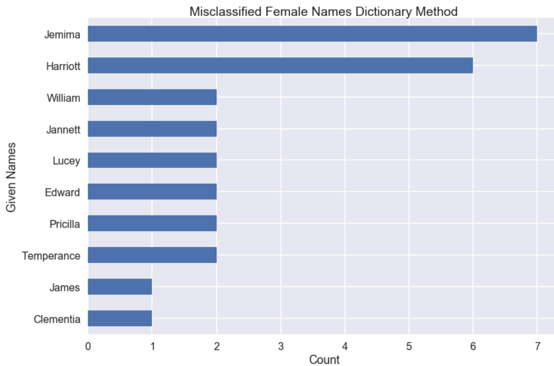
Figure 8. Dictionary-based female misclassifications
