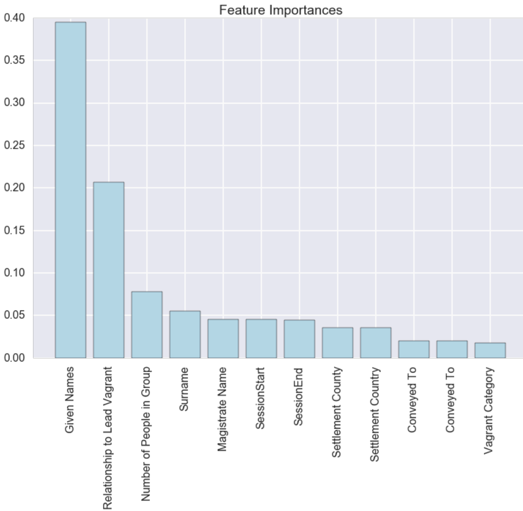
Figure 12. Feature importance random forest
