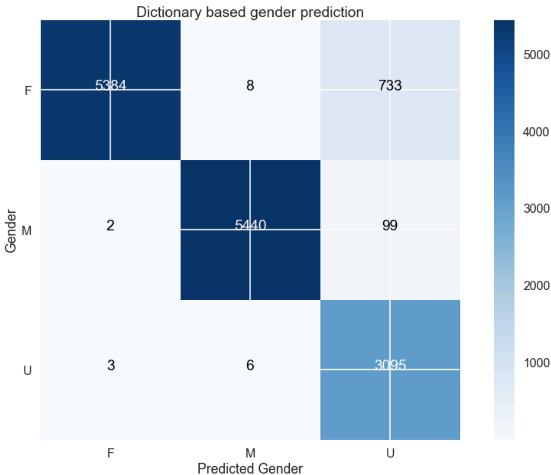
Figure 7. Confusion matrix dictionary-based gender prediction
